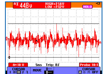
Without AEGIS® SGR: 44.8 V peak-peak
