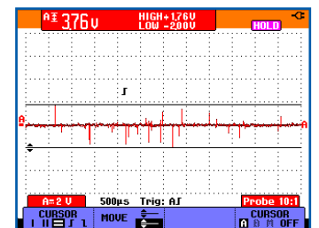
With AEGIS® SGR: 3.76 V peak-peak
